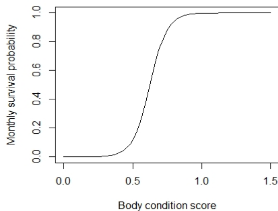
Figure A1.5: Relationship between body condition and monthly survival probability. The maximum monthly survival probability is set at 0.99, to reflect an annual background survival probability of 0.88
